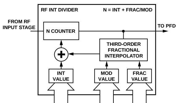
Figure 20. RF INT Divider
